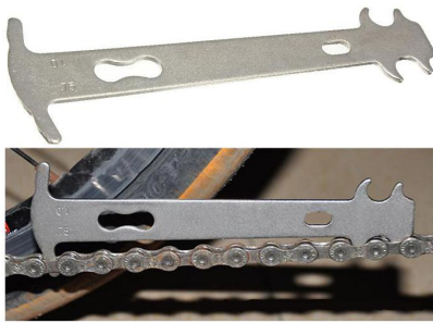
9724L Chain wear indicator
