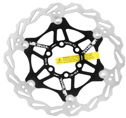
Snail disc rotor Material: Aluminium alloy Size: 160/180/203mm Hole distance:44mm Thickness:1.8mm Color:black,red,blue,green, purple gold
