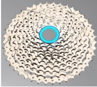
11S Cassette Sprocket Model: CS1142 Ratio: 11T-42T Finish: CP, Nickel Packing: 30 pcs/ctn
