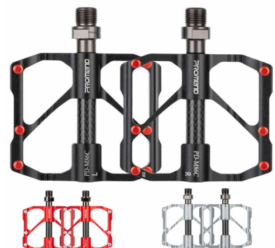
R86C Alloy bike pedal 114x94x 295g/Pair 9/16"
