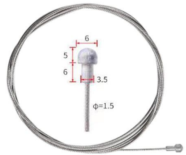
Road bike brake cable 1700mm
