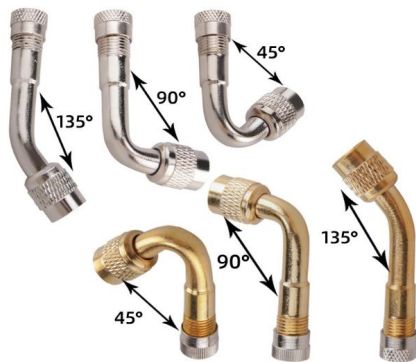
Brass Valve extender Material: Copper Color: Silver, gold Size: 45°/90°/135°
